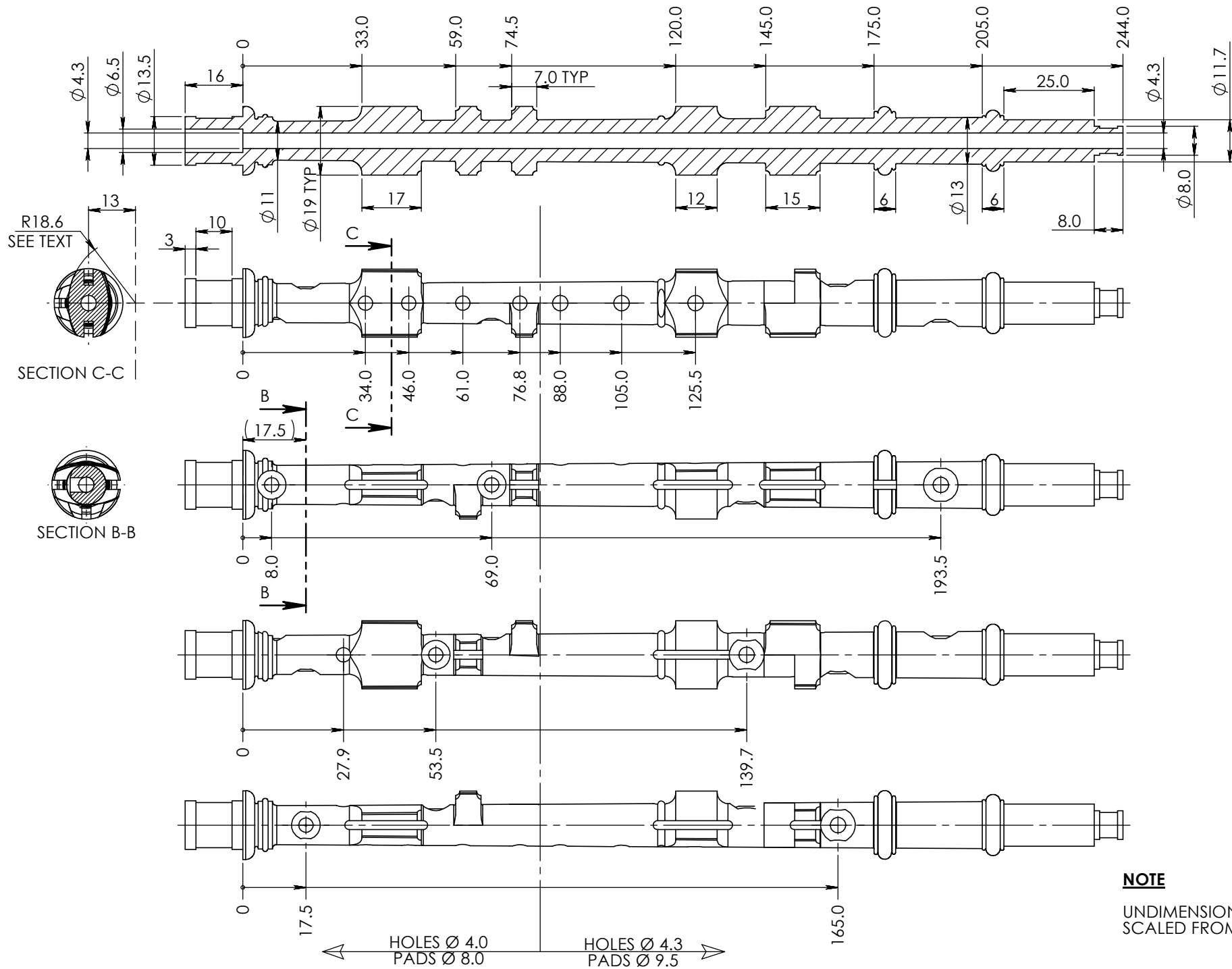
STANDARD 7 KEY CHANTER TO PLAY AT CONCERT "G" PITCH
